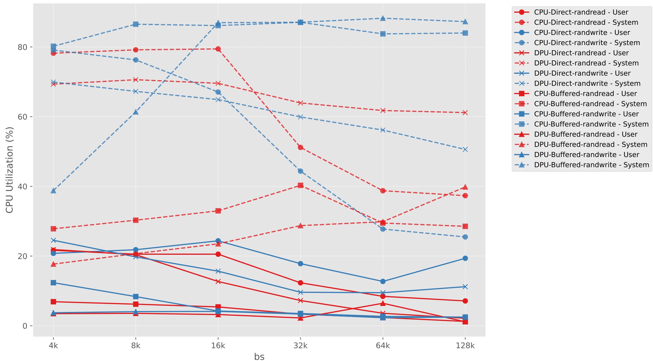
CPU Utilization vs bs (CPU vs DPU, Direct vs Buffered)
